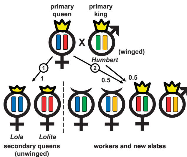
Figure 3. The mixed mode of reproduction as observed in the termites R. speratus and R. virginicus [1, 10], in which new queens are produced clonally (1, r = 1 to their mother), via automictic parthenogenesis and terminal fusion [1], but workers and new alates are produced sexually (2, r = 0.5 to their mother and father). Note that even with incestuous mating, common in termites, this system does not result in a significant decrease in heterozygosity. Imagine, for example that Lola and Lolita each mate with their father Humbert after the primary queen dies, and that both replace her (in these species, many secondary queens can co-occur within the same colony, [1]). In that case, the new worker and alate offspring that Lola and Lolita produce would have roughly the same heterozygosity as those produced by the primary queen and king [1]. This is because the secondary queens are produced asexually, and so do not share any genes with their father.
