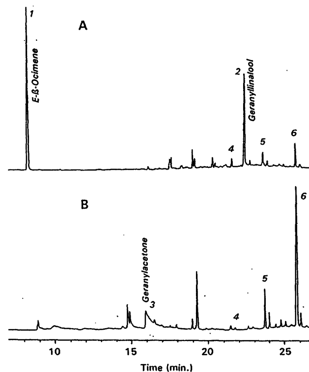
FIG. 2. Total ion chromatograms of the two different patterns seen in the secretions of Dufour glands of soldiers of Eciton burchelli : (A) one dominated by ( E )- \beta -ocimene (peak 1) and geranylinalool (peak 2), and (B) one where these are replaced by geranylacetone (peak 3); other peaks are nonadecane (4), heneicosene (5), and tricosene (6).
