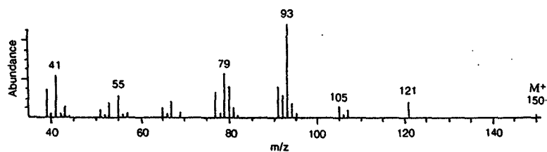
FIG. 4. Mass spectrum of the minor compound in the Dufour glands of Labidus praedator , identified as homooximene.
