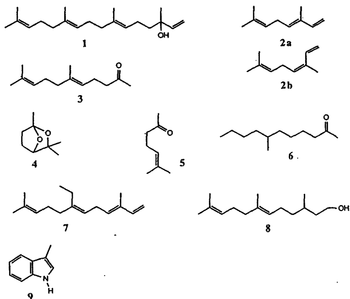
FIG. 1. Chemical structures: 1, geranylinalool; 2a, ( E )- \beta -ocimene; 2b, ( Z )- \beta -ocimene; 3, geranylacetone; 4, 1,3,3-trimethyl-2,7-dioxabicyclo[2.2,1]heptane; 5, 6-methyl-5-hepten-2-one; 6, 7-methyl-2-undecanone; 7, ( E,E )- \alpha -homofarnesene; 8, 2,3-dihydrofarnesol; 9, skatole.
