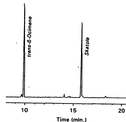
FIG. 3. Total ion chromatogram of the volatile compounds in a whole gaster of a worker of L. praedator . A Dufour gland chromatographed under the same conditions showed only one peak for β-ocimene.
