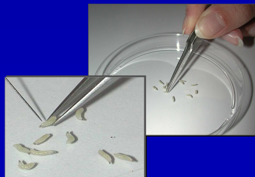
MALDI-TOF MS
